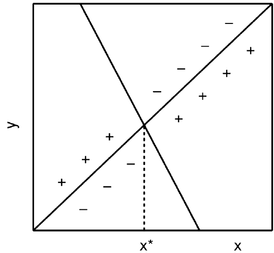
Fig. 5 A pairwise invasibility plot, where mutant phenotypes are denoted by y and resident phenotypes by x . The diagonal corresponds to the line y = x . The point of intersection of the two solid lines, corresponds to x = x^* and at this point there is a vanishing fitness gradient: D(x^*) = 0 . The point, x^* is termed an 'Evolutionarily Singular Strategy'.
